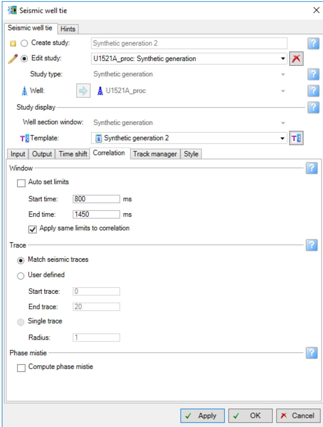
Figure 6: Correlation tab
