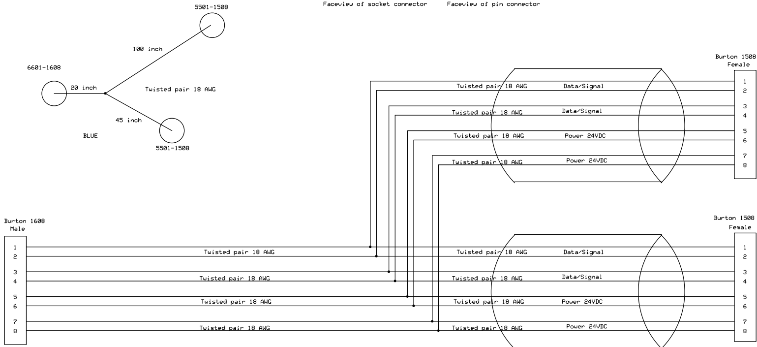
Faceview of socket connector
