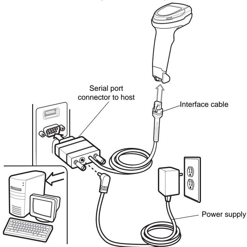
Figure 6-1 RS-232 Connection
