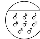
Faceview of pin connector
