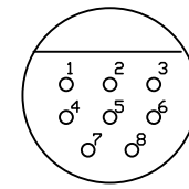
Faceview of socket connector
